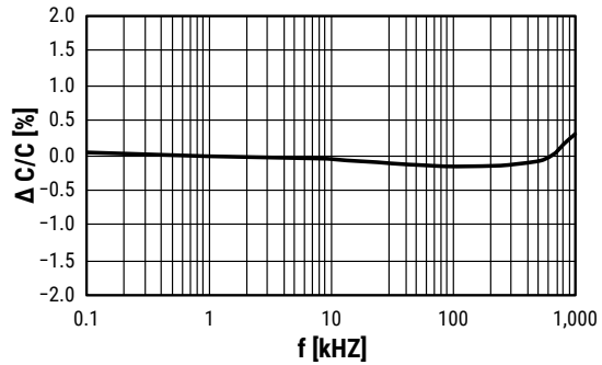
Dissipation Factor vs. Frequency
