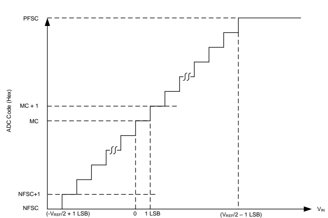
Figure 44. Ideal Transfer Characteristics for Pseudo-Differential Configuration
