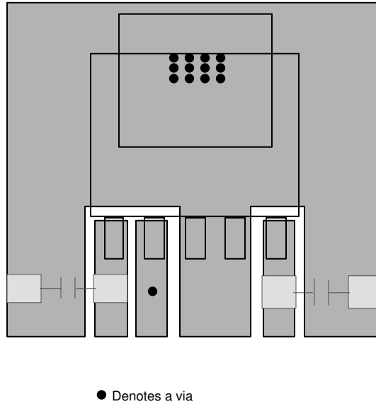
Figure 10-2. KVU Package Fixed Output
