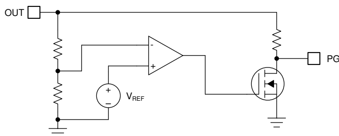
Figure 7-4. Simplified Power-Good Schematic
