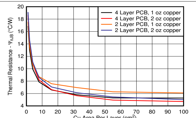
Figure 8-5. \psi_{JB} vs Copper Area (KVU Package)
