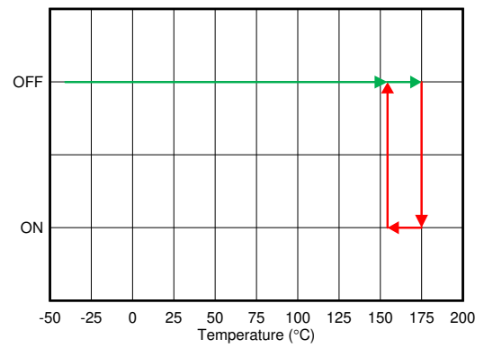
Figure 6-38. Thermal Shutdown
