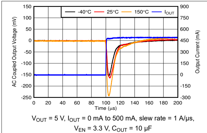
Figure 6-25. Load Transient, No Load to 500-mA Rising Edge
