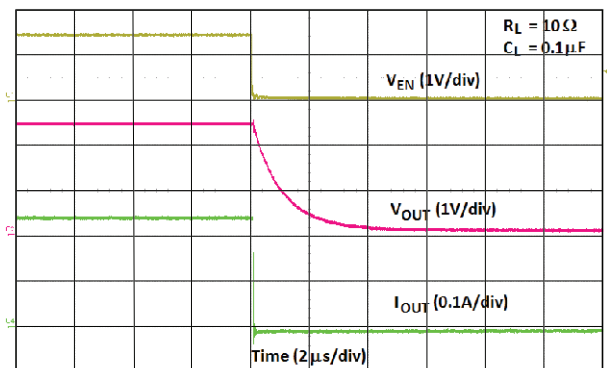
Fig. 26 - Turn-Off Time ( V_{IN} = 2.5\text{ V} )
